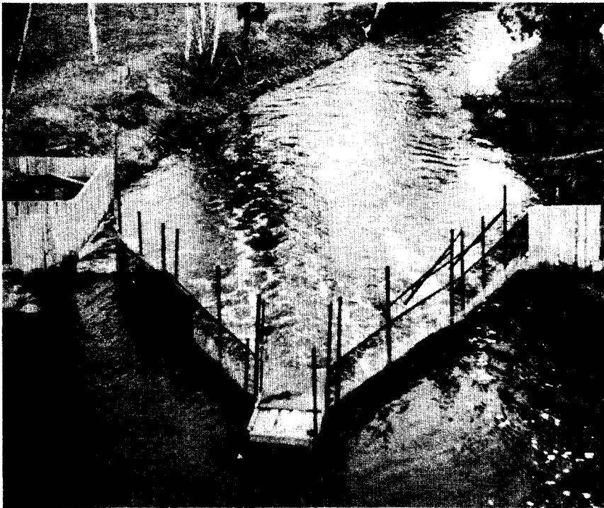
Figure 9.--Carp Creek weir, May 5, 1947. Looking downstream.
