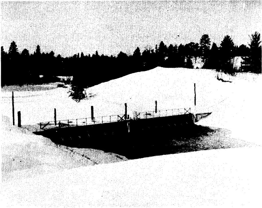
Figure 58.--Ocqueoc River sea lamprey weir and traps during operation in winter months. February, 1949. (View from downstream.)
