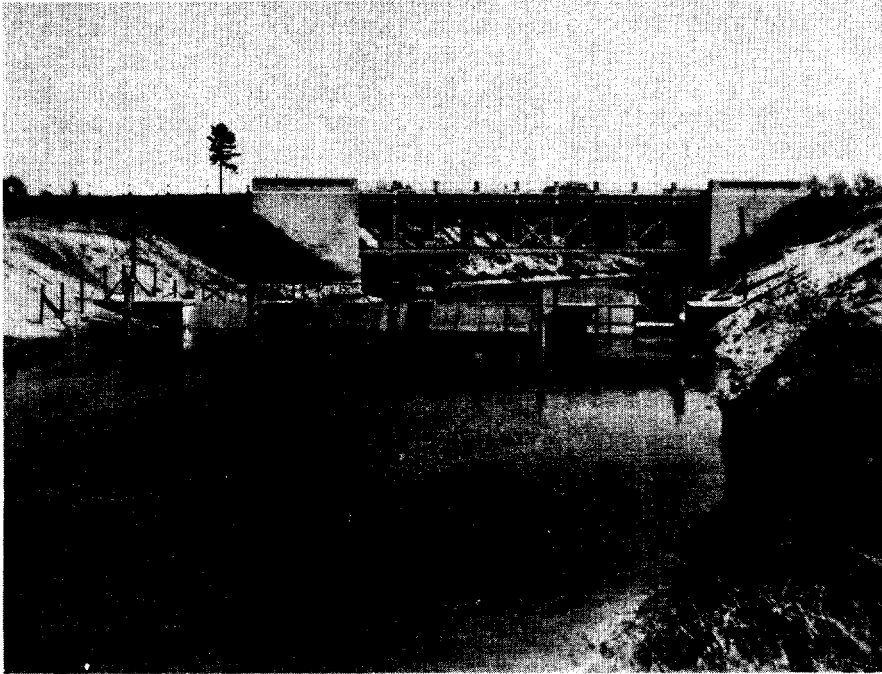
Figure 12.--Ocqueoc River sea lamprey weir. View from upstream.
